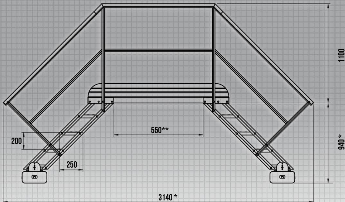
SIDE VIEW
